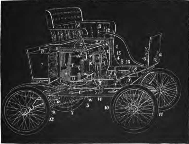
FIG. 245.—Diagram of the "Locomobile" Steam Carriage, showing parts in position. A is the boiler shell of copper; a, the winding of steel piano wire; B, the double cylinder engine; C, the adjustable strut, or distance rod; D, the compensating gear; E, pipe leading from engine to muffler, F, for exhaust steam; G, pipe leading from muffler to vent at H; I, the water supply tank; J, feed pump operated from the engine cross-head; K, cock in front of check valve on water supply pipe, for cutting off the supply from the tank; L, pipe leading from pump to the by-pass, M; N, lever for operating the by-pass; O, fuel supply tank; P, reserve air tank; Q, the dashboard; R, the air-pressure gauge; S, pipe leading from fuel tank to burner, through which gasoline is passed under air pressure; T, metal straps holding the lagging, U, around the boiler; A; V, the diaphragm fuel feed regulator, explained in connection with Fig. 207; W, pipe leading steam from boiler to diaphragm of the regulator; X, the water glass; Y, the mirror for reflecting the water glass; Z, starting lever. Other parts are: The crank arm on Z acting on the lever (1); the reversing lever (2); crank arms on the reversing lever (3 and 4); the pop safety valve set at 240 pounds (5); the steam pressure gauge (6); fuel valve to main burner (7); foot pedal (8) operating band brake (9); wire wheel spokes (10); pneumatic tire (11); steering handle (12); sprocket on rear axle (13); blow-off valve (14); oil feed cup on engine cylinders (15); pipe from air tank to fuel tank (16).
